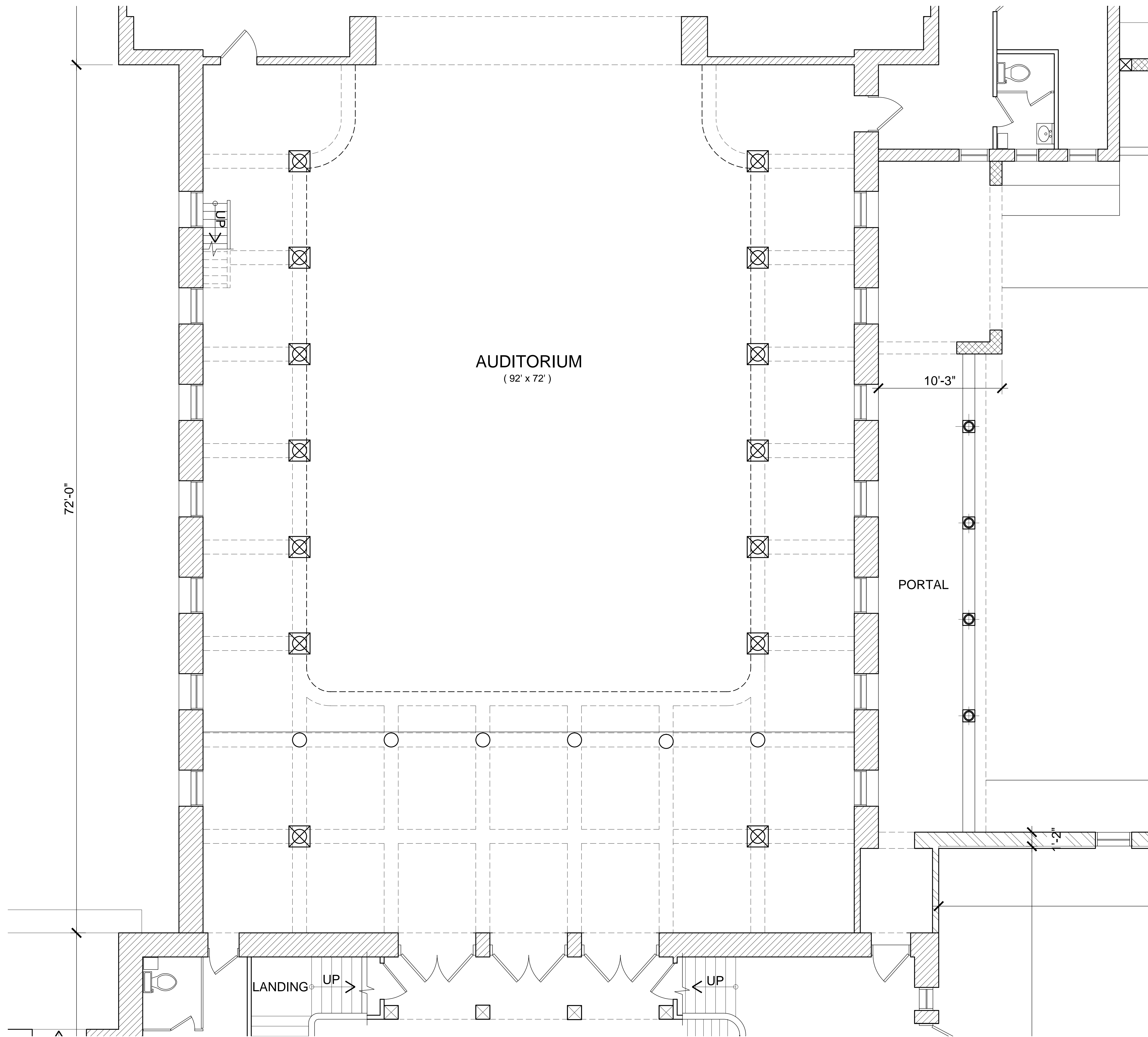
(A) AUDITORIUM SCALE: 1/4" = 1'-0"
